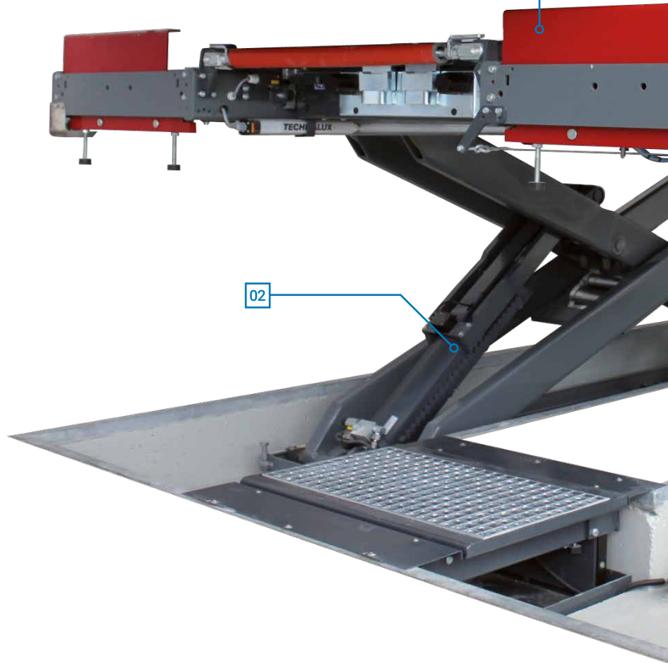
High-powered drive unit – designed for extremely large number of lifting cycles.
