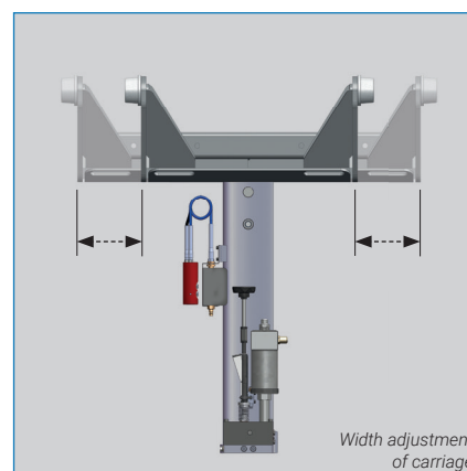
Pit jack with P-carriage and support system
